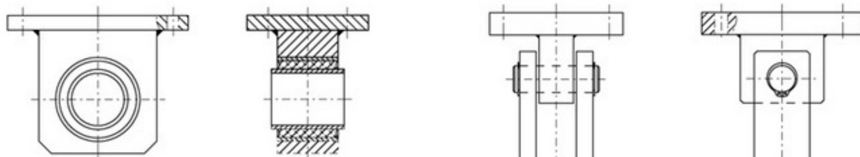
齿轮箱摇摆支点支座 Supports for gear unit swing-bases
